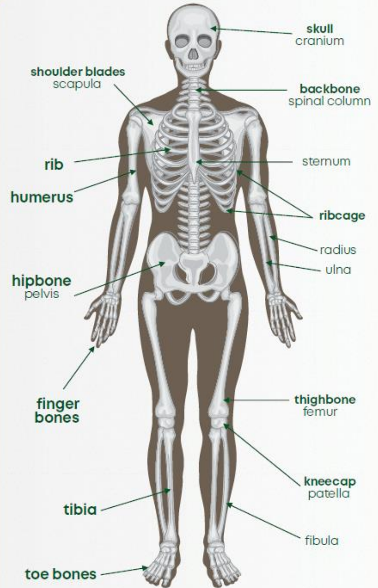
SKELETAL SYSTEM
