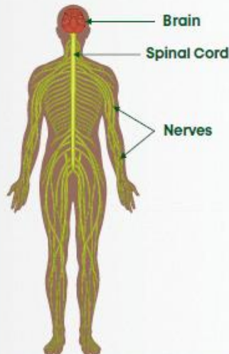
NERVOUS SYSTEM
