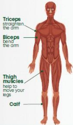
MUSCULAR SYSTEM
