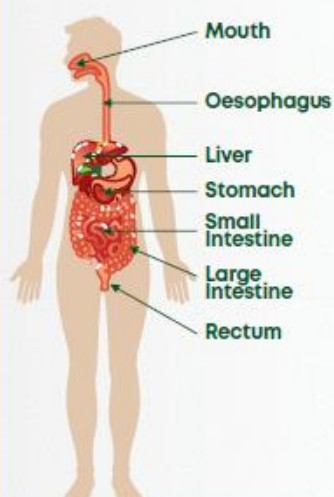
DIGESTIVE SYSTEM
